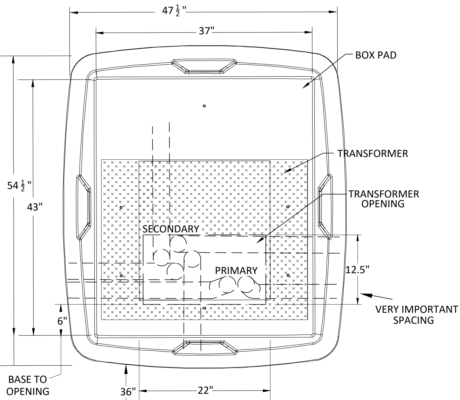
TOP VIEW
