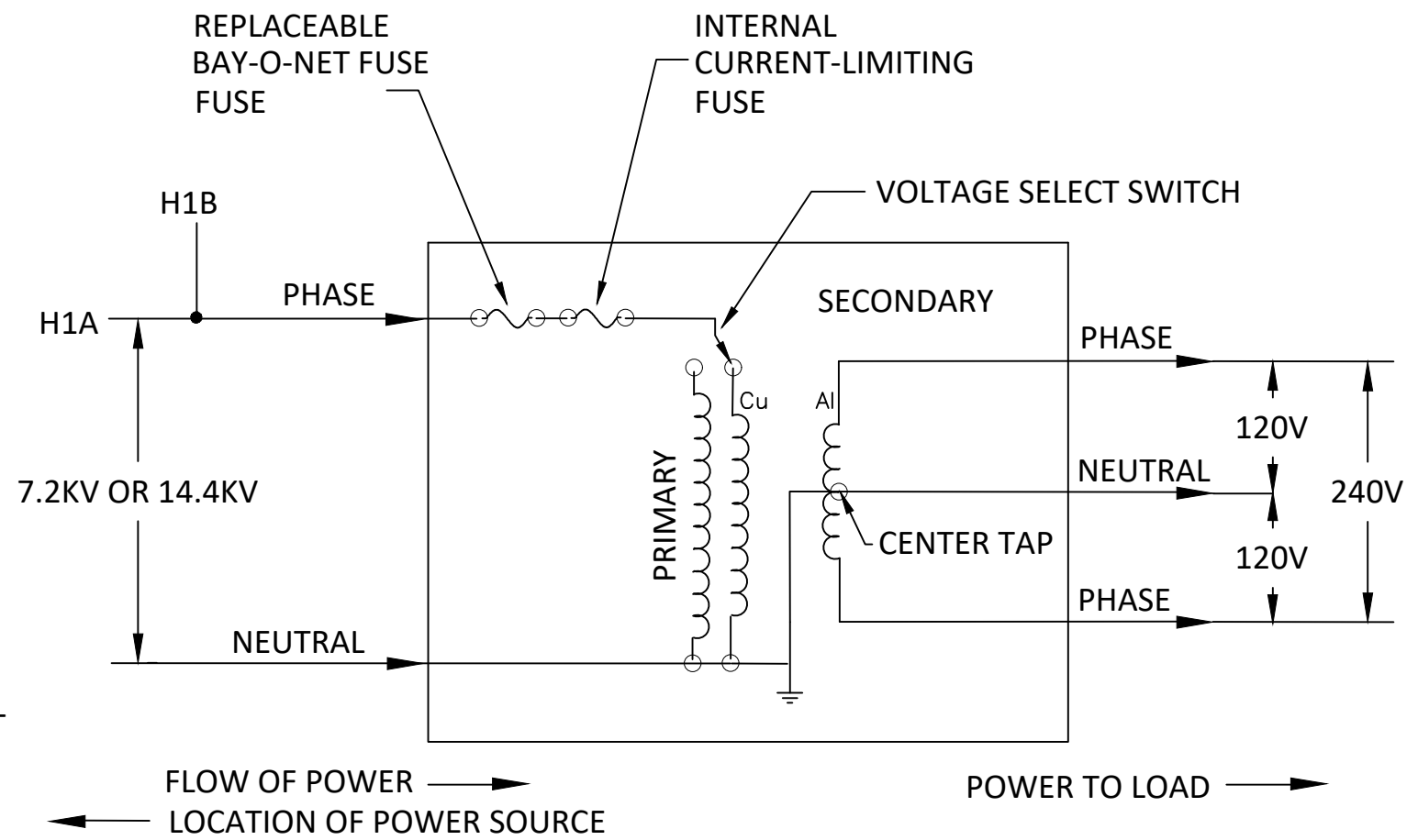
WIRING DIAGRAM
