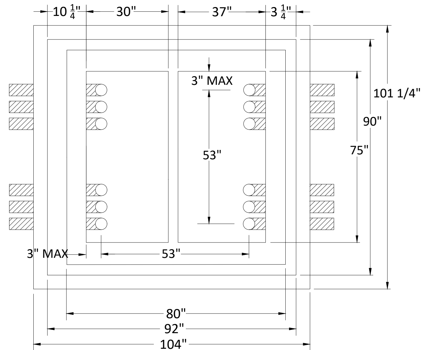
TOP VIEW
