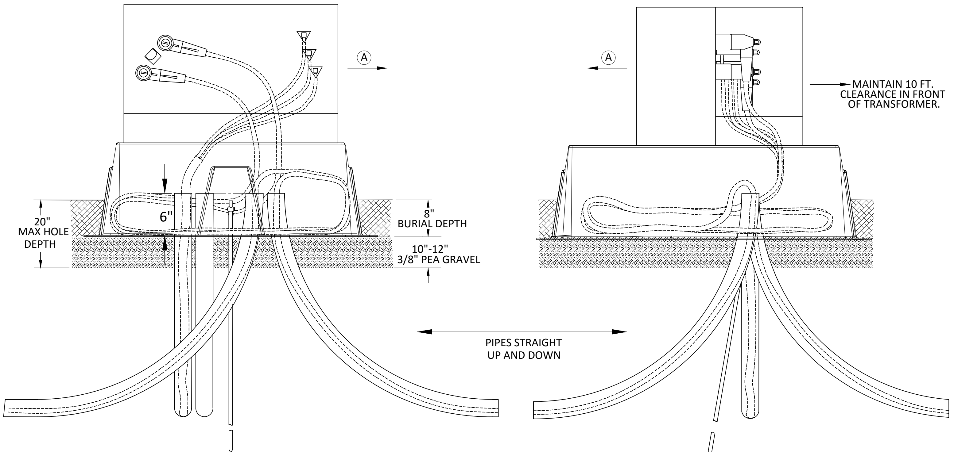
FRONT VIEW
